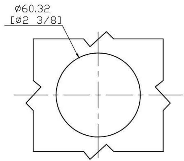
PANEL PREPARATION
